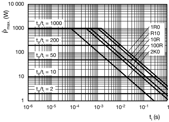
AC01 and AC01-AT Pulse on a regular basis; max. permissible peak pulse power ( \hat{P}_{max} ) as a function of pulse duration ( t_i )
